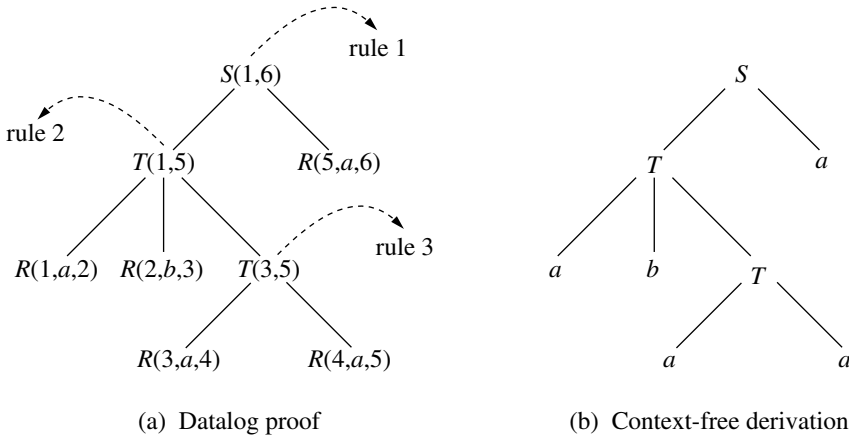
Figure 12.3: Proof tree
