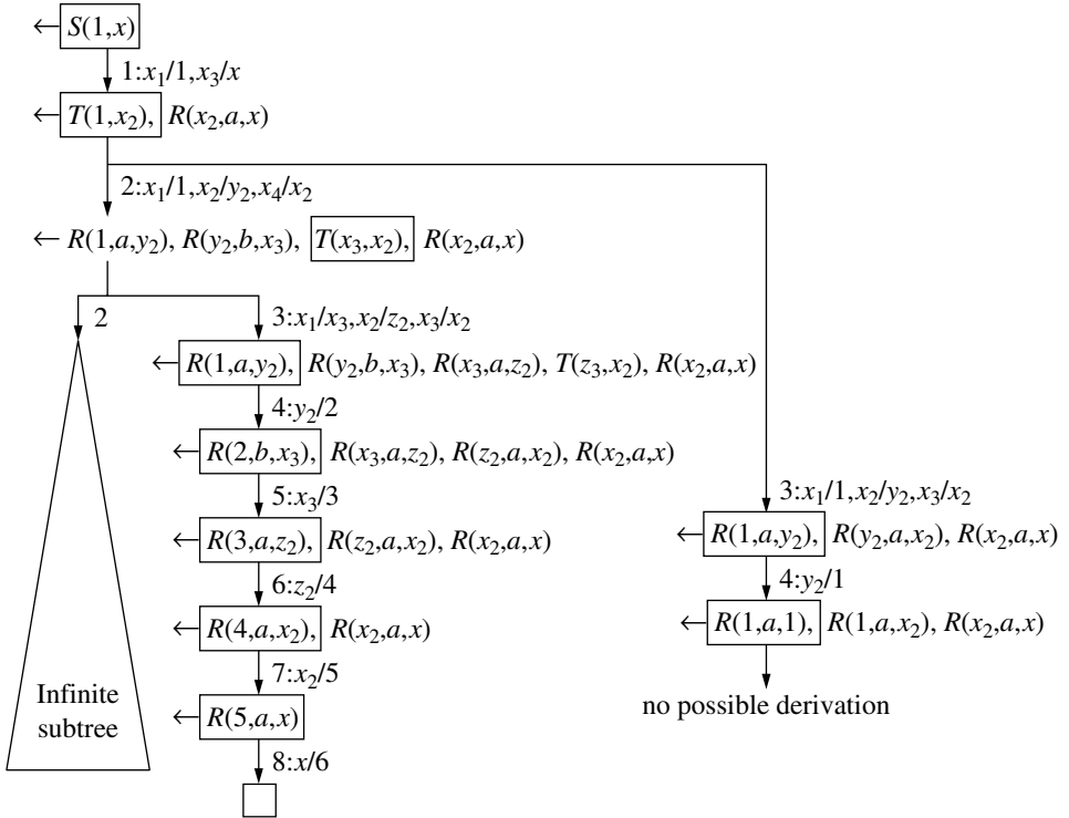
Figure 12.6: SLD tree
