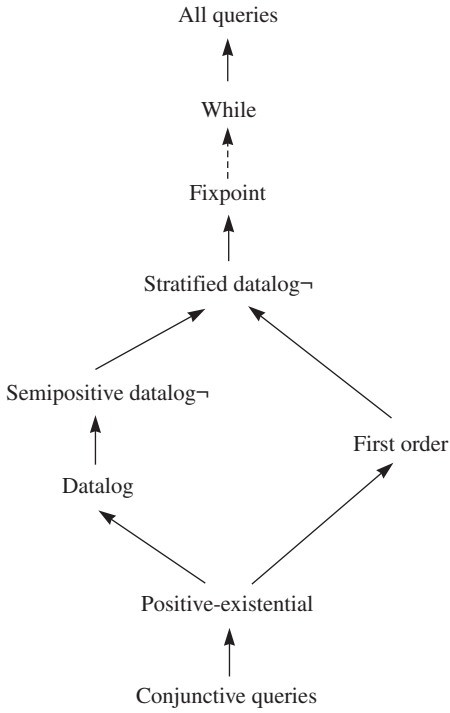
Figure 18.4: Main classes of queries
