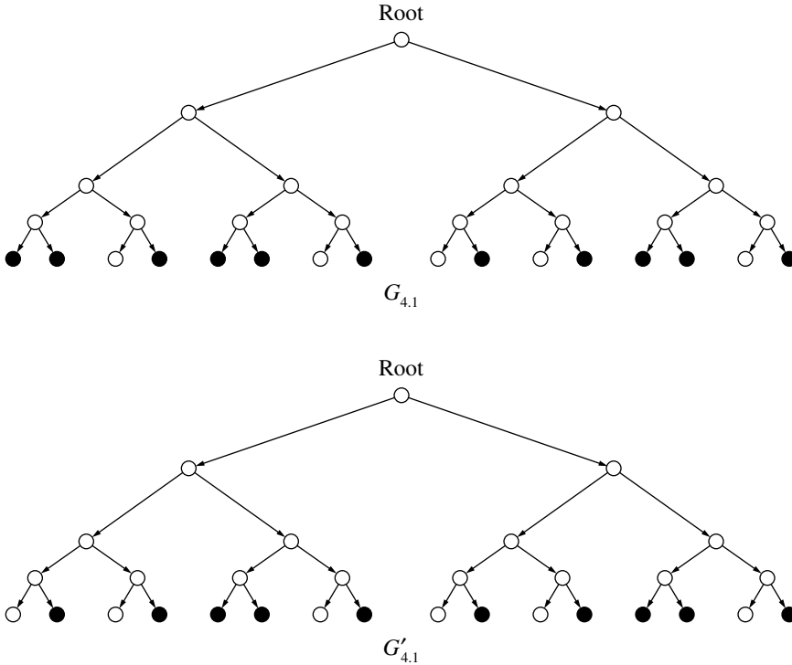
Figure 15.2: Game trees
