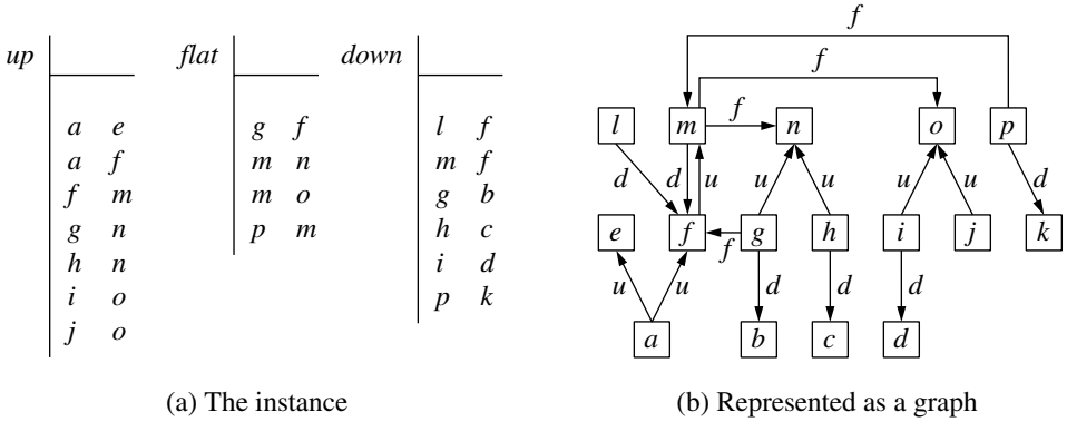
Figure 13.1: Instance \mathbf{I}_0 for RSG example
