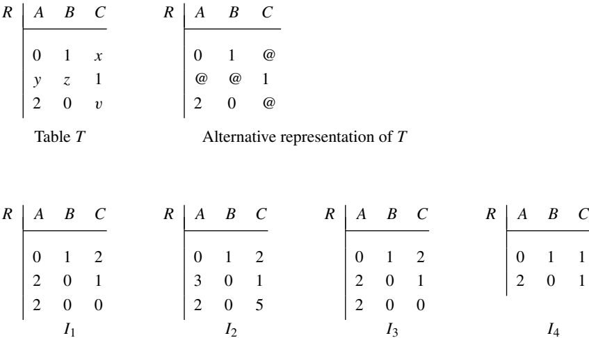
Figure 19.1: A table and examples of corresponding instances
