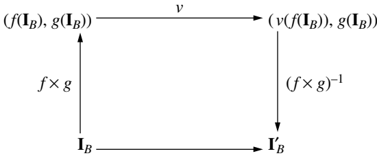
Figure 22.2: Properties of a g -translation \mu of view update v on view f
