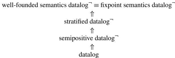
Figure 15.3: Relative expressive power of datalog (¬) languages
