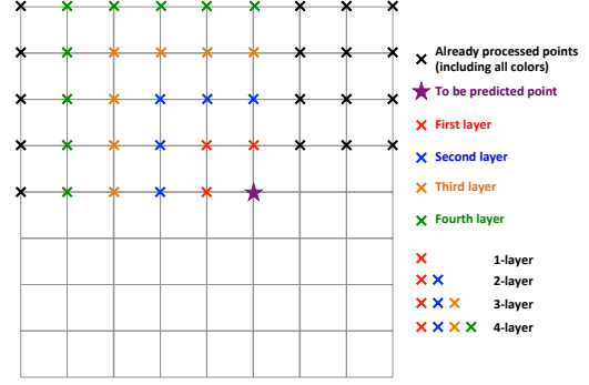
Figure 1. Example of 9 \times 9 two-dimensional data set showing the processed / processing data and the data in different layers of the prediction model.
