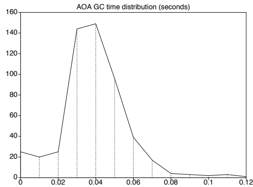
Figure 3: Pause distribution, compiler run
