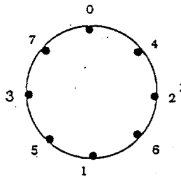
Figure 4: A symmetric ring of size 8
