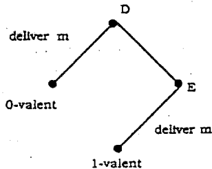
Figure 3: Neighboring configurations D and E leading to configurations of opposite valence
