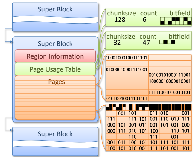
Figure 1: Overview of the data structures used in the ScatterAlloc : Memory is organized in super blocks which are collected in a list. Each super block holds a fixed number of equally sized pages, information about the usage of each page and meta information collected for regions of pages. The usage table captures the size according to which the page is split into equally sized chunks, the counter of used chunks and a bit field to identify the used chunks. To allow for splitting the page into more chunks than actually can be captured by the bit field in the usage table, an additional hierarchy of bits is placed on the beginning of the page.
